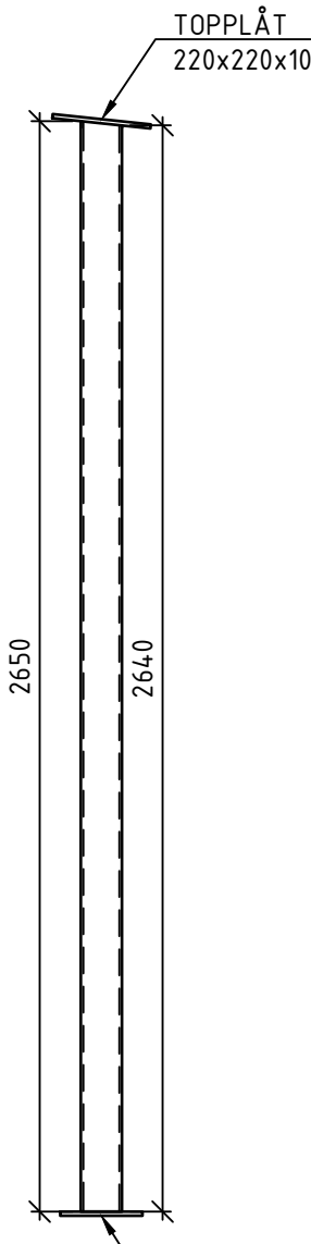
SP01d 1:20 VKR 100x100x6.3 ANTAL: 1st
