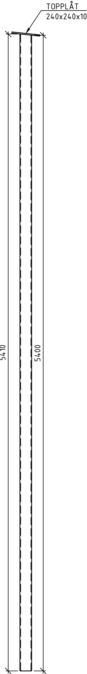
SP01a 1:20 VKR 100x100x6.3 ANTAL: 1st
