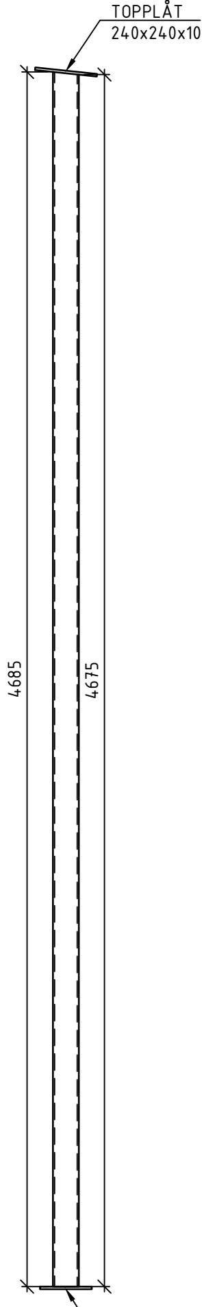
SP01b 1:20 VKR 100x100x6.3 ANTAL: 1st
