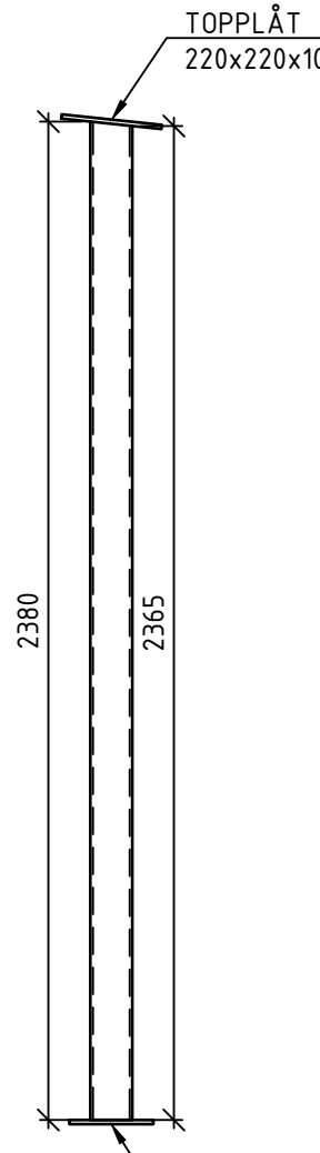
SP01e 1:20 VKR 100x100x6.3 ANTAL: 1st
