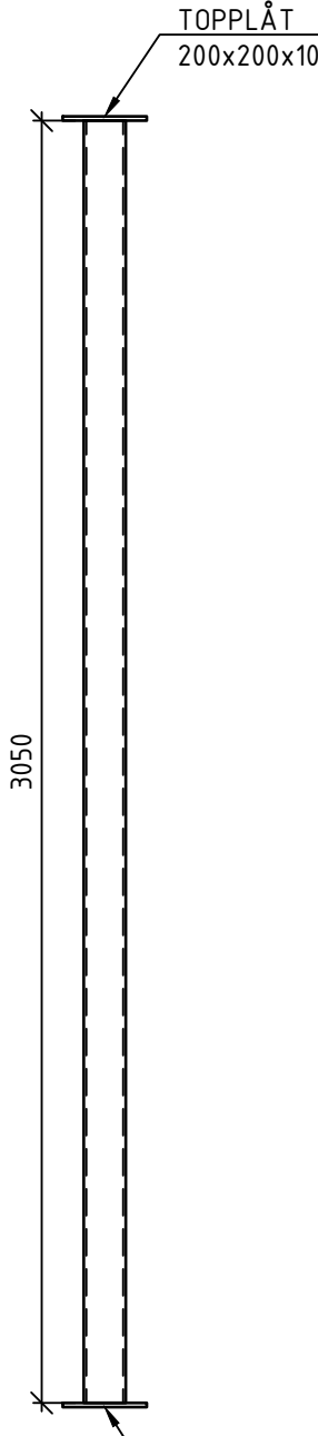
SP01c 1:20 VKR 100x100x6.3 ANTAL: 4st
